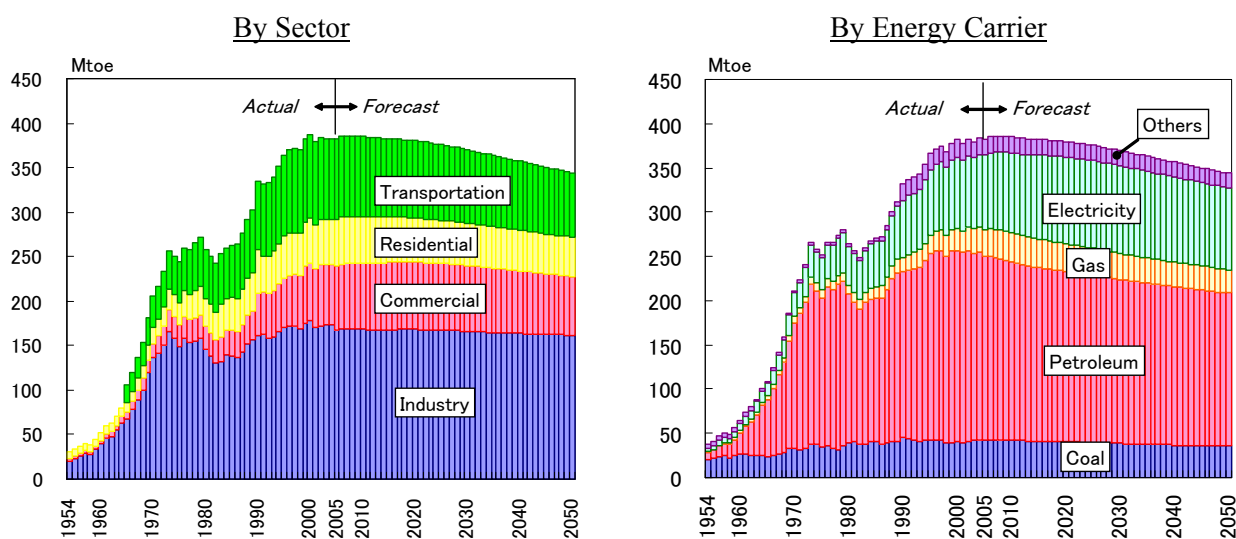
Figure 5.1: Final Energy Demand
