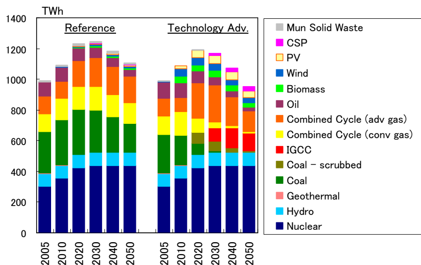
Figure 6.1: Power Generation Mix
