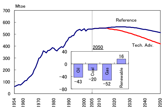
Figure 6.5: Primary Energy Supply
