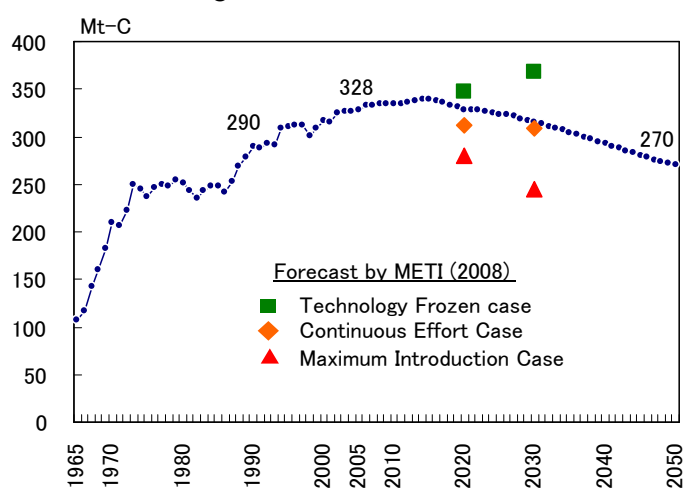
Figure 5.3: CO 2 emissions
