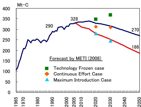
Figure 6.7: CO 2 emissions
