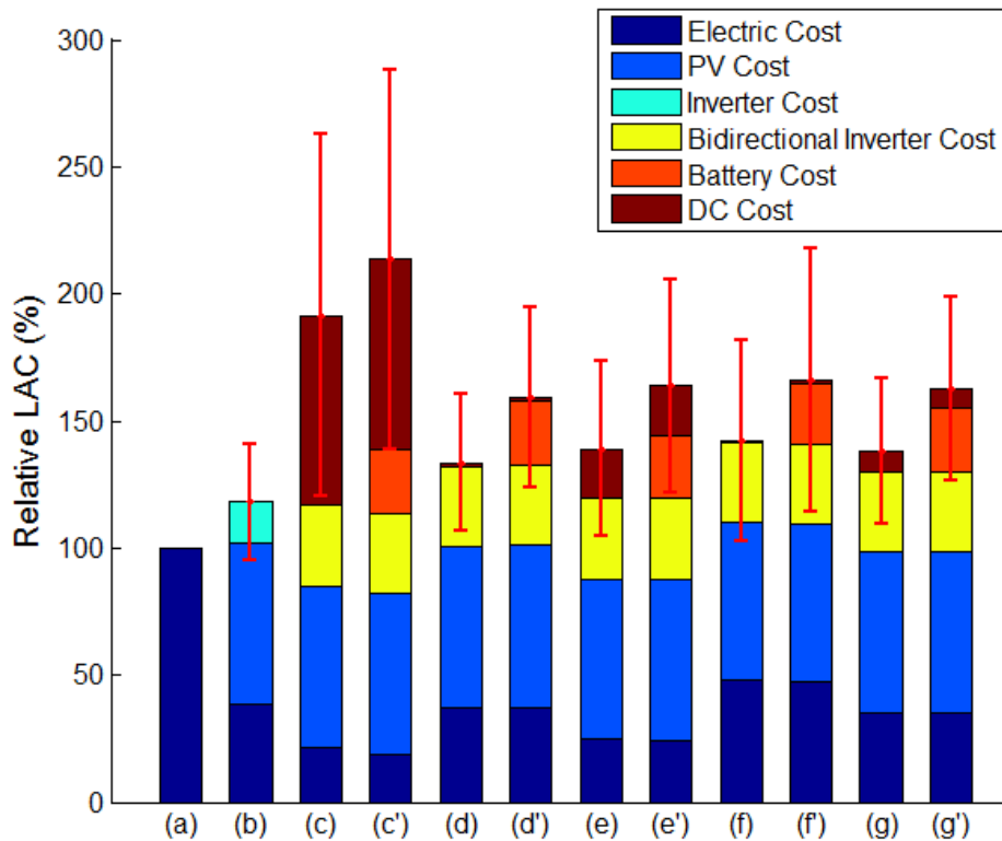
Figure 4. Levelized annual costs for the systems shown in Figure 2(a) through Figure 2(g). Primes indicate results with battery storage for solar generated energy. Results are shown as a percentage of a traditional (AC) home with no PV generation's annual electric bill. Bars show the mean result for each simulation. Error bars show plus or minus one standard deviation from the mean.
